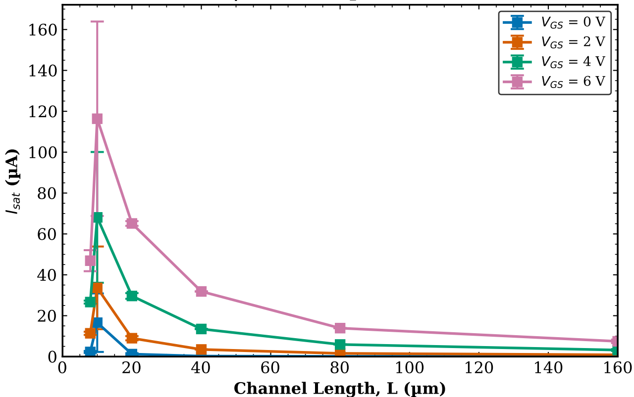
TFT1 Combined (Tr. 1 & 2) I_{sat} vs L | W = 100 \mu\text{m} (mean \pm std)
